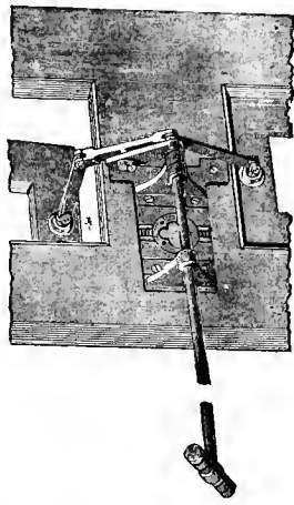
Fig. 4331. One Window Open. MANSFIELD DECK-SASH OPENER.
